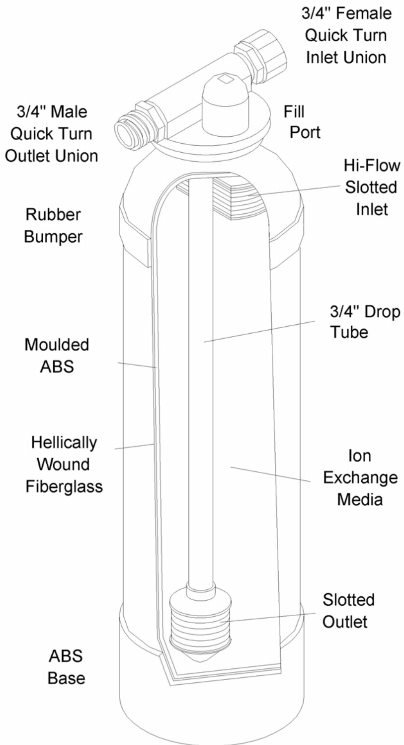
724-FG Series Service Deionizer Tank
